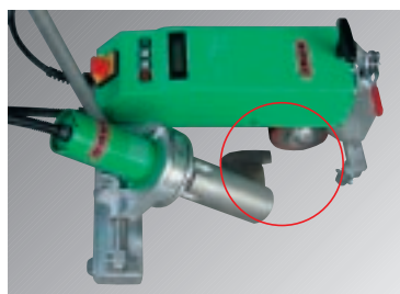
Welding seam width 20 mm
